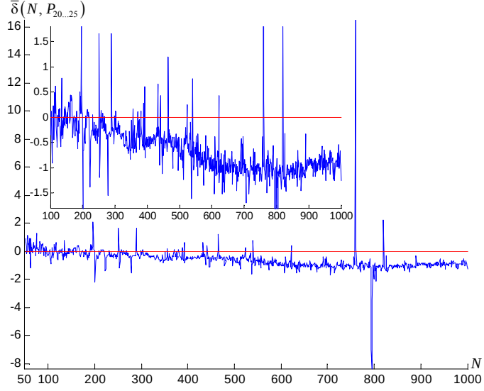
Fig. 7. AE (32) over graphs in Fig. 6. The additional graph ignores artifacts.
