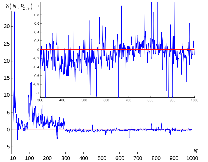
Fig. 3. AE (31) over graphs in Fig. 2. The additional graph ignores artifacts.
