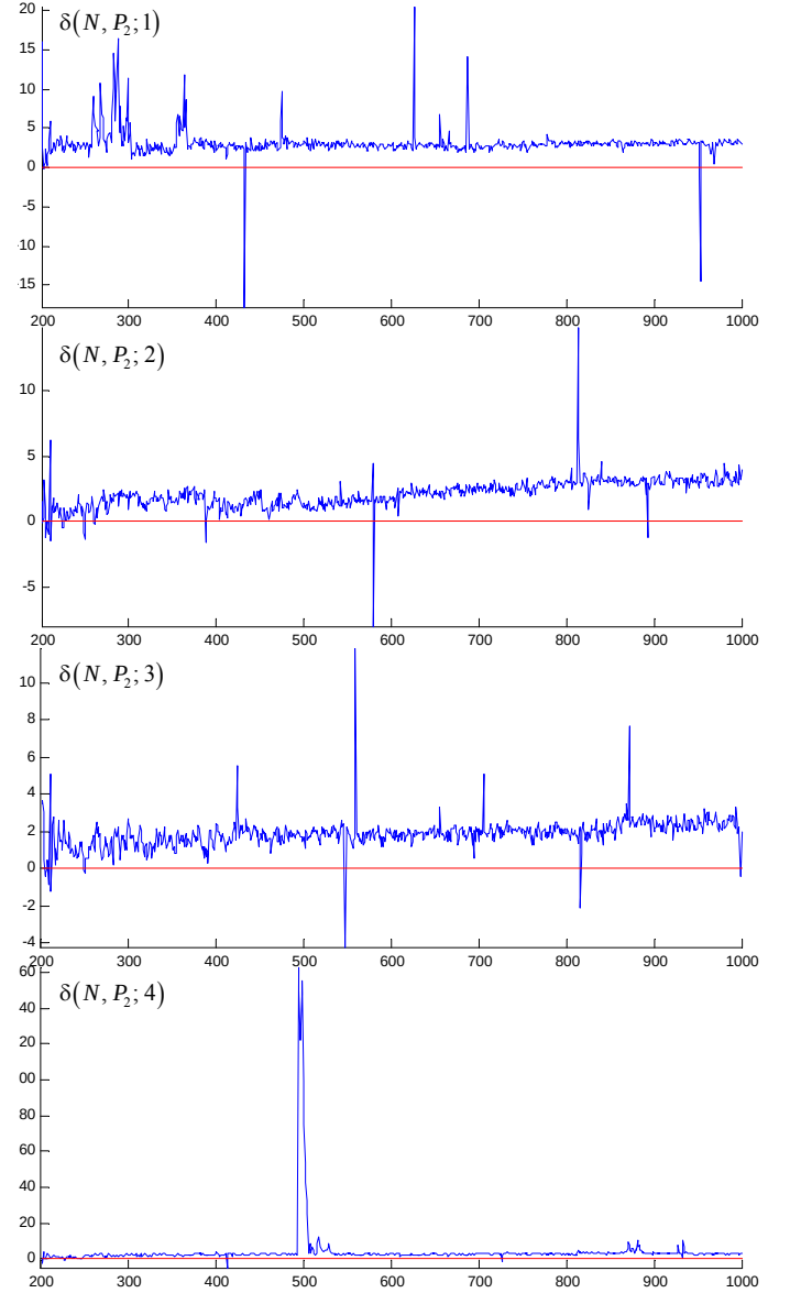
Fig. 9. The DJOI gain (with uncut artifacts) in scheduling “smoother” PPJSPs, wherein jobs of the “smoother” PPJSPs are of 5 and 6 parts, whereas PPJSPs generated by the smallest additional parameter in (30) are of 2 and 3 parts.
