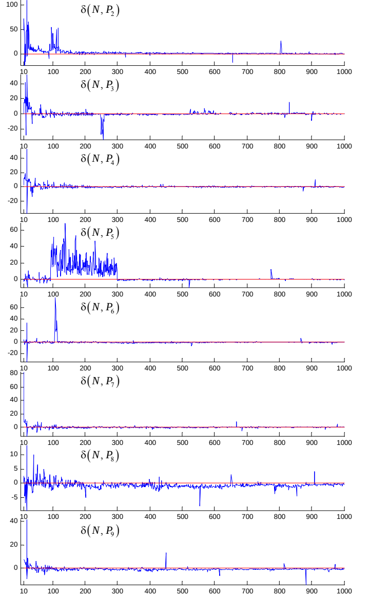
Fig. 2. Estimators (24) over 100 PPJSPs, where artifacts are not cut. Artifacts are essential for a few hundreds of jobs due to the shorter computation time.
