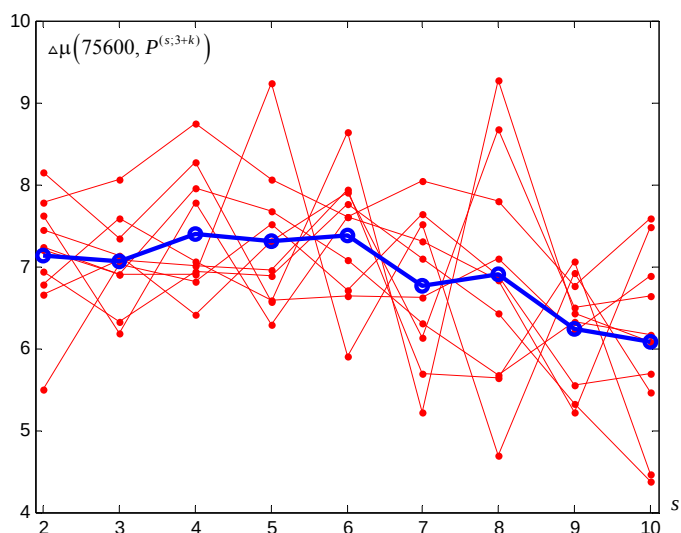
Fig. 13. The difference between AJOI and DJOI computation times in seconds for the set of 10 estimators in Fig. 12 (the average is the thicker line with circles). While the decreasing of the DJOI relative advantage is quite certain, the “steeper” PPJSPs herein are still solved by 6 seconds faster with DJOI.
