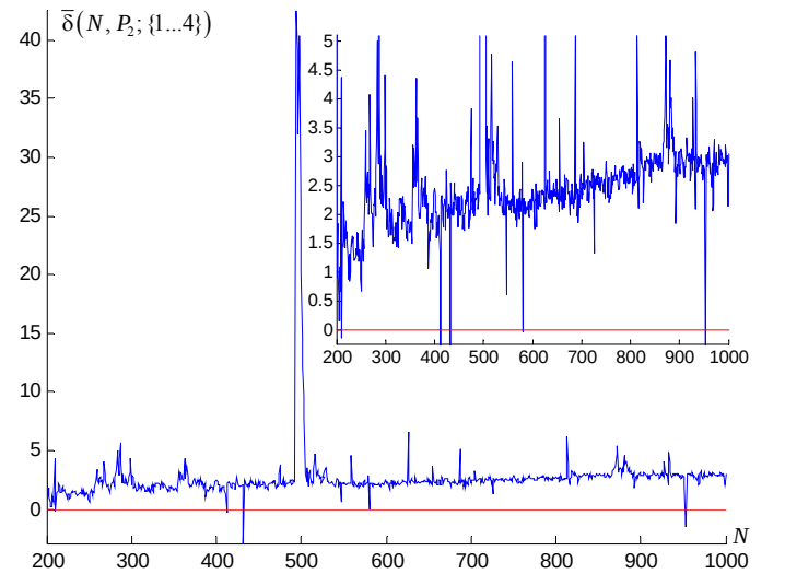
Fig. 10. AE (33) over graphs in Fig. 9. The relatively huge artifact is cut in the additional graph. An increase of the AE is seen in the additional graph.
