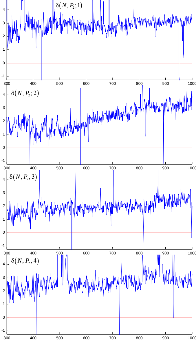
Fig. 11. The zoom-ins on the 4 graphs of Fig. 9 without their minor artifacts. The slight increase of the DJOI gain is clearly seen (the abrupt increase for k_{\text{smooth}} = 2 is an artifact of the increase trend itself). It is also seen that solving such PPJSPs for 1000 jobs and more is sped up by almost 3 % with DJOI.
