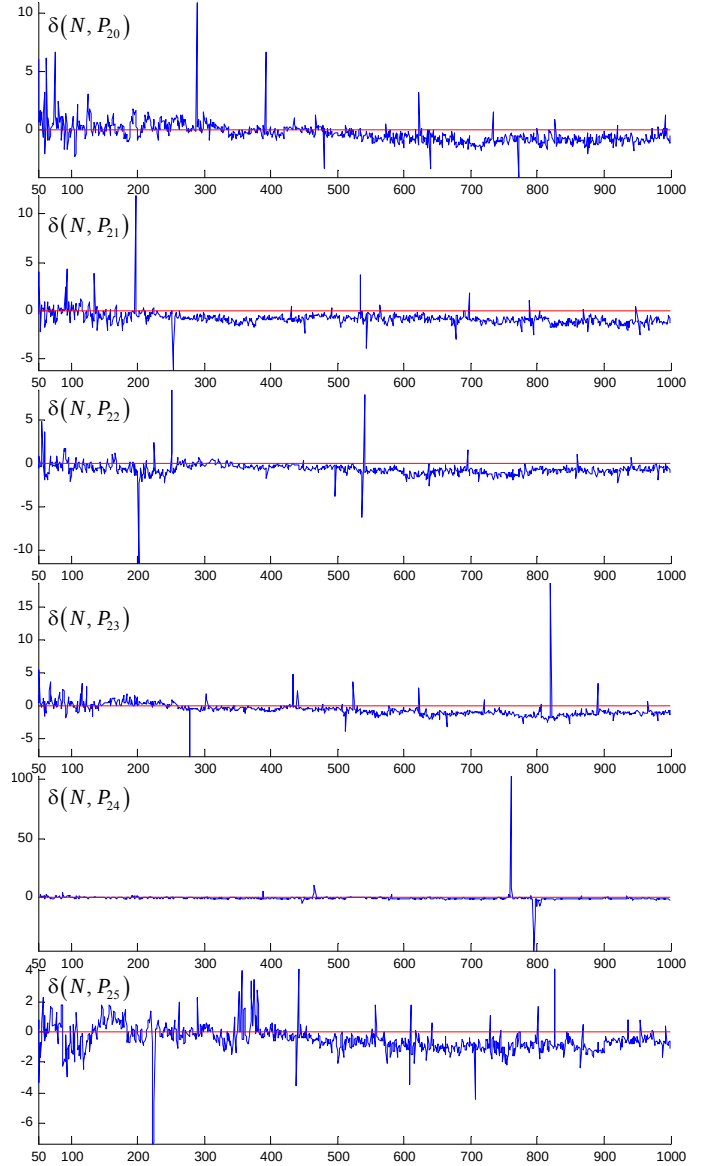
Fig. 6. Estimators (24) over 100 “steeper” PPJSPs, wherein jobs are of greater volumes than job volumes in Fig. 5, with uncut artifacts. Artifacts are lesser compared to those ones in Fig. 2 because here the computation time is longer.
