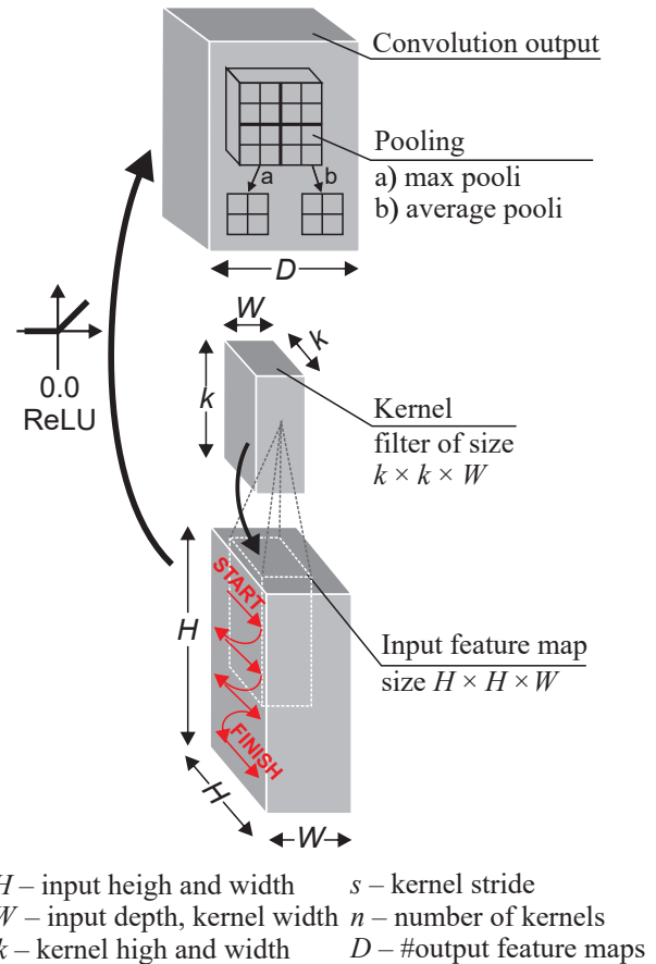
Fig. 1. The convolution process.
