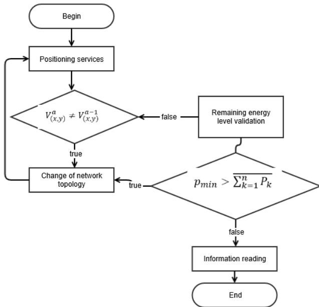
Fig. 2. The algorithm of the performance pertaining to the network agent.
