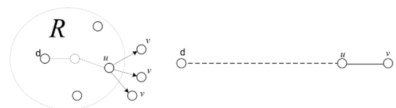
Fig. 4. Applying Dijkstra's algorithm.
